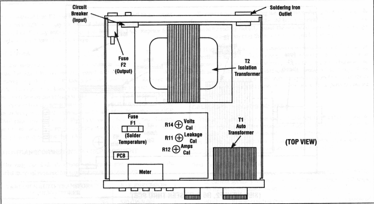
Figure 14. Location of Fuses and Calibration Adjustments, Model 1420.
