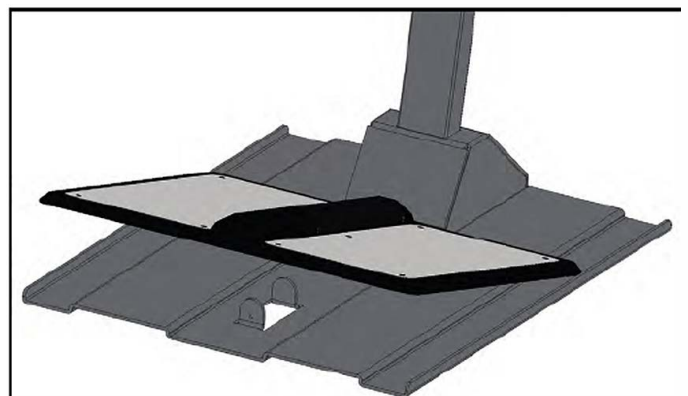
Figure 7. Installing the dual foot plate onto the baseplate
