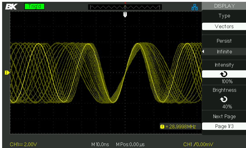
Figure 3.36 – Persist Screen
