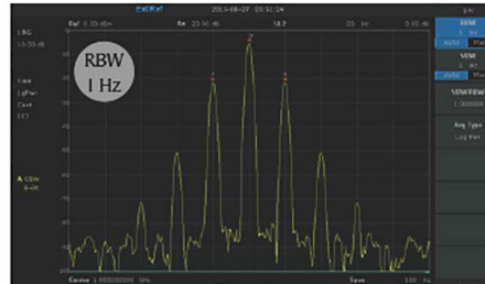
Low resolution bandwidth helps differentiate between adjacent signals
