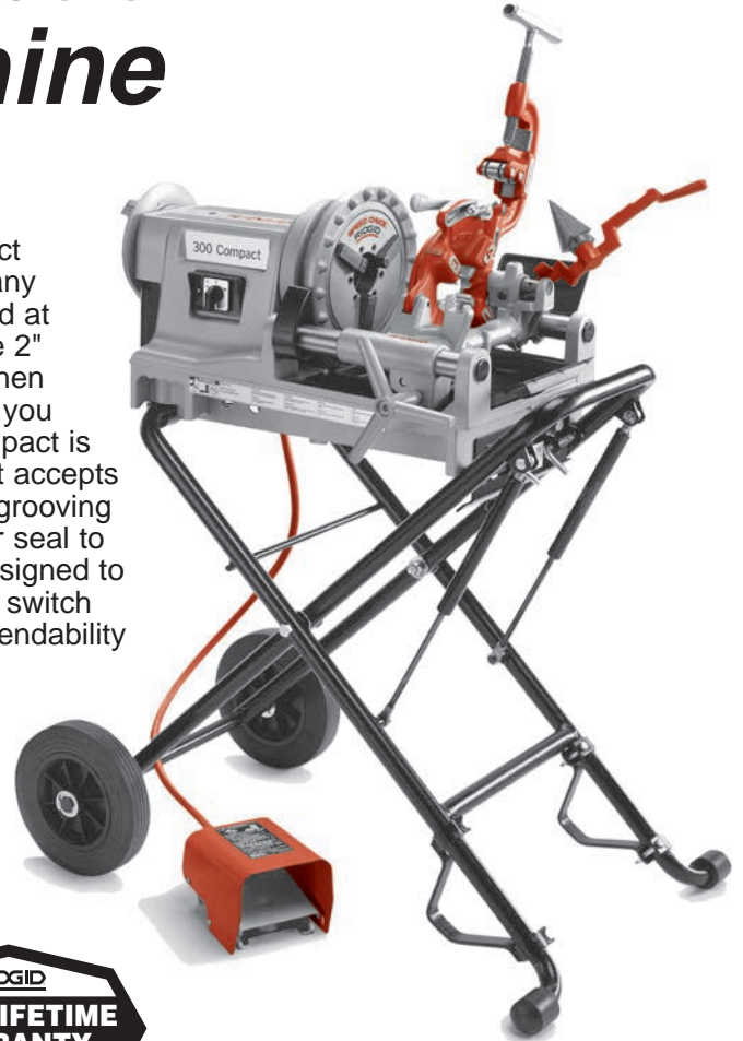
300 Compact shown with optional Model 250 Folding Wheel Stand
