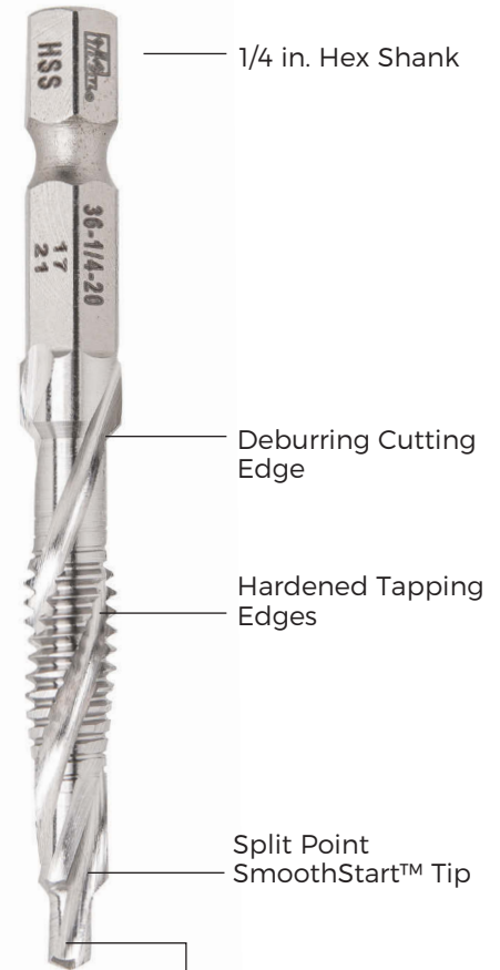
3-flute Design
