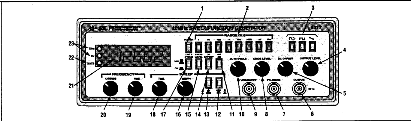
Figure 1. Model 4017 Front Panel.
