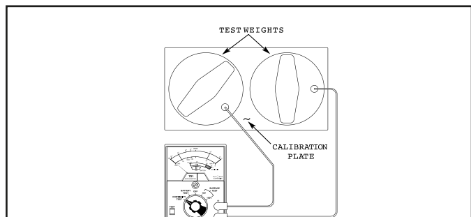
Figure 3. Analog Surface Resistance Megohmmeter Kit, continuity test.
