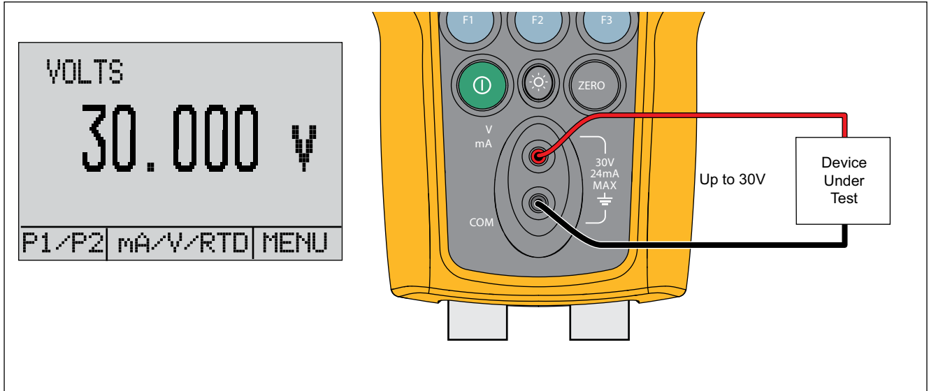
Figure 7. Voltage Measurement
