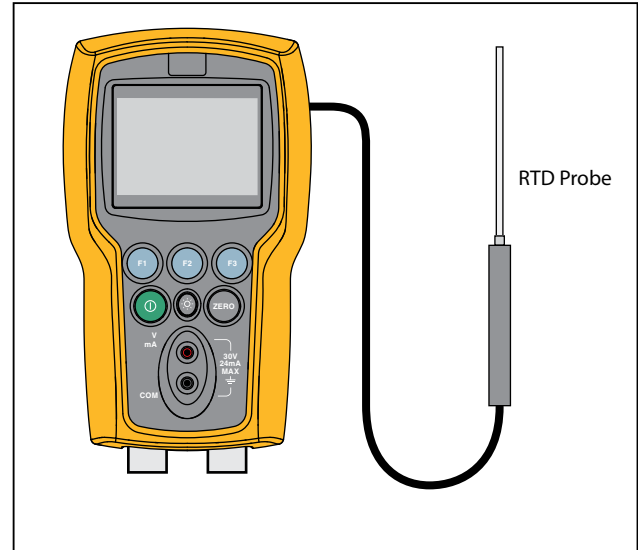
Figure 5. Temperature Measurement with RTD Probe
