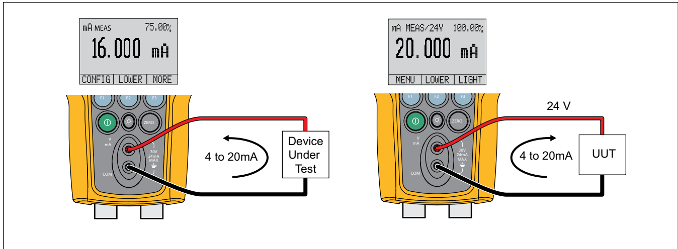
Figure 6. Measure Current
