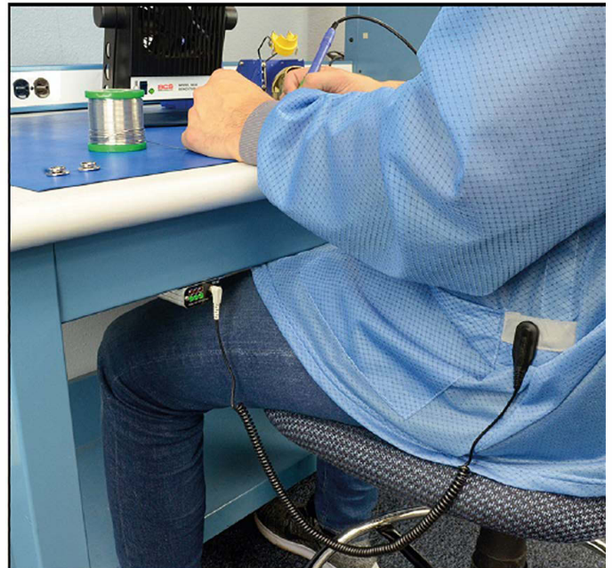
Figure 6. Using the Dual-Wire Static Control Smock with the SCS CTC331-WW Iron Man® Plus Workstation Monitor
