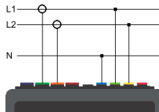
Split-phase 3 wires (L1, L2, and N)
