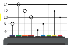
Three-phase 5 wires (L1, L2, L3, N, and earth)
