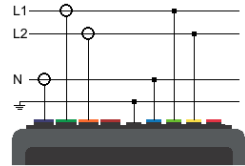
Split-phase 4 wires (L1, L2, N, and earth)
