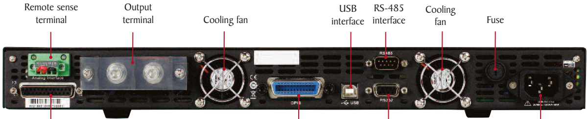
Models 9115 / 9115-AT / 9116
