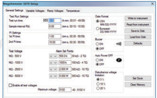
Four tabbed dialog boxes allow for clear and easy setup of all functions of the Model 5070, including setup for variable voltage and alarm set points, as well as step voltage tests and temperature compensation.
