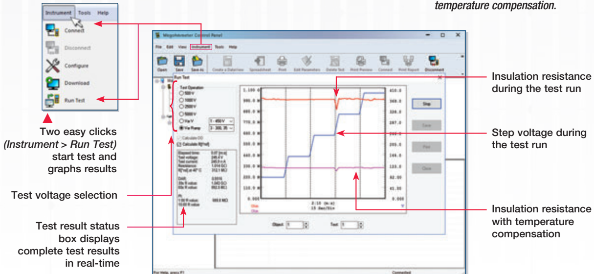
Run test and display text and graphical results from one dialog box. Model 5070 also displays step voltage.
