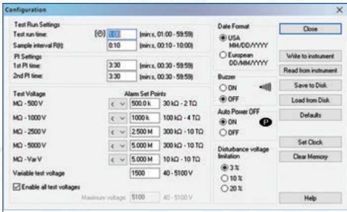
Configuration screen allows you to set alarm levels, test time and to read and write configurations from and to the instrument.
