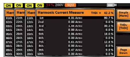
Current Harmonic
