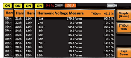
Voltage Harmonic
