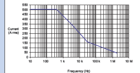
Maximum Input Current vs. Frequency
