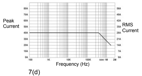
Figure 7(a – d): Maximum Current versus Frequency
