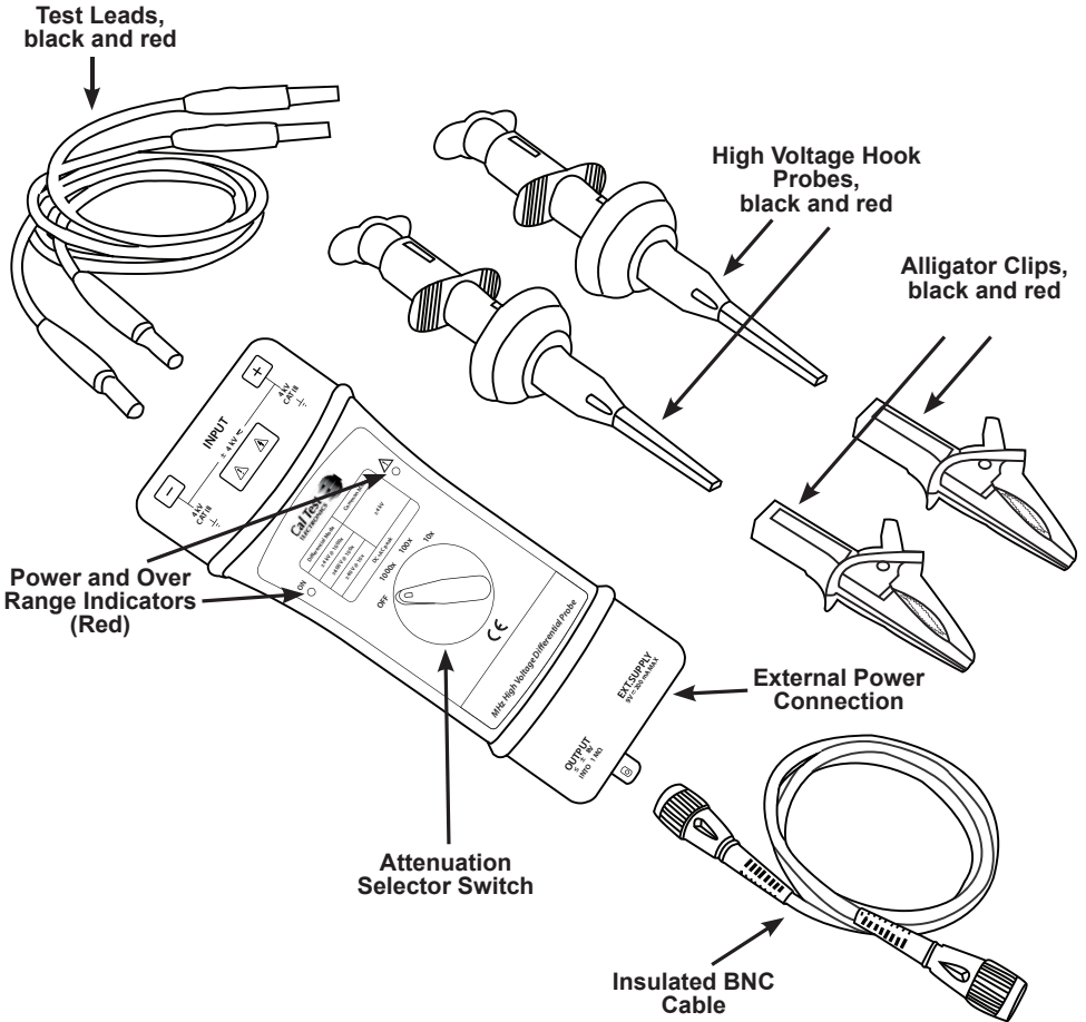
Figure 1 Front Panel Features
