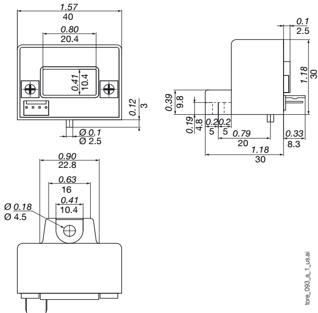
Solid-core sensors 50 ... 600 A (frame size 1)
