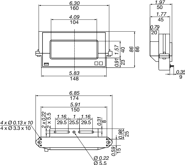
Split-core sensors 800 ... 2000 A (frame size 2)
