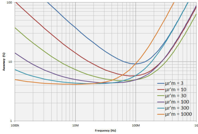
Figure 45. Permeability accuracy ( \frac{\Delta\mu'}{\mu'_r} ) vs. frequency (at F = 0.5 mm, typical)
