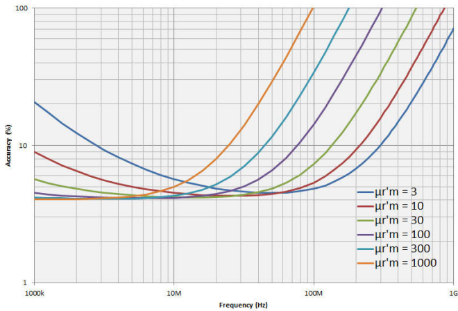
Figure 47. Permeability accuracy ( \frac{\Delta\mu'}{\mu'_r} ) vs. frequency (at F = 10 mm, typical)
