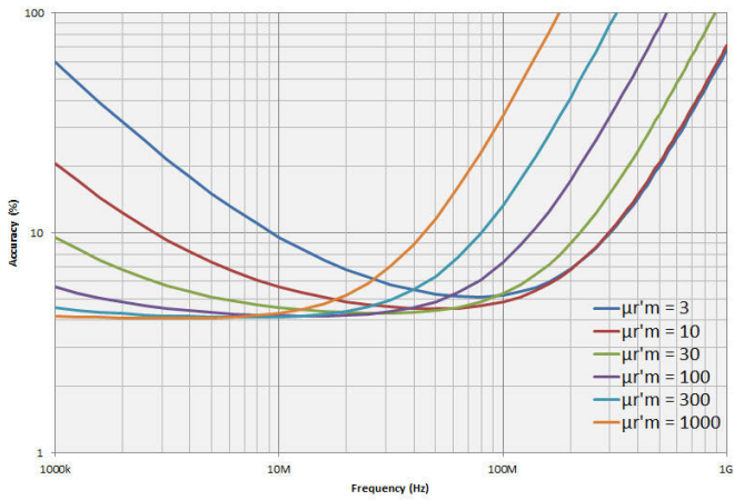
Figure 46. Permeability accuracy ( \frac{\Delta\mu'}{\mu'_r} ) vs. frequency (at F = 3 mm, typical)
