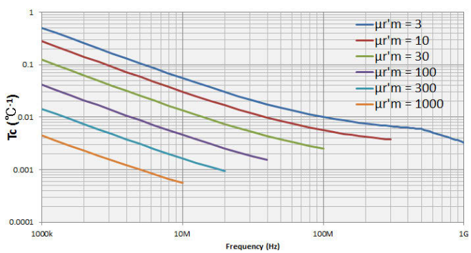
Figure 58. Typical frequency characteristics of temperature coefficient of \mu_r' (at F = 3 mm)
