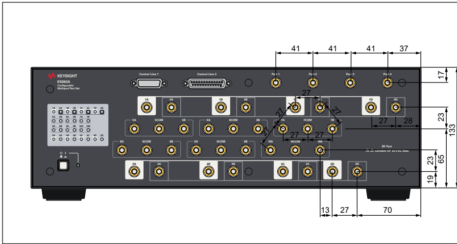
Figure 11. Dimensions (pitch between switches, with Option E5092A-020, in millimeters, nominal)
