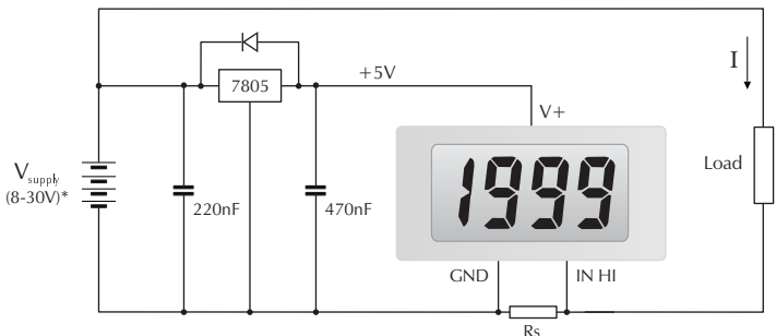
Measuring current.
