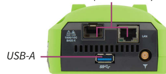
Main Ethernet Test Ports (RJ-45 & SFP)
