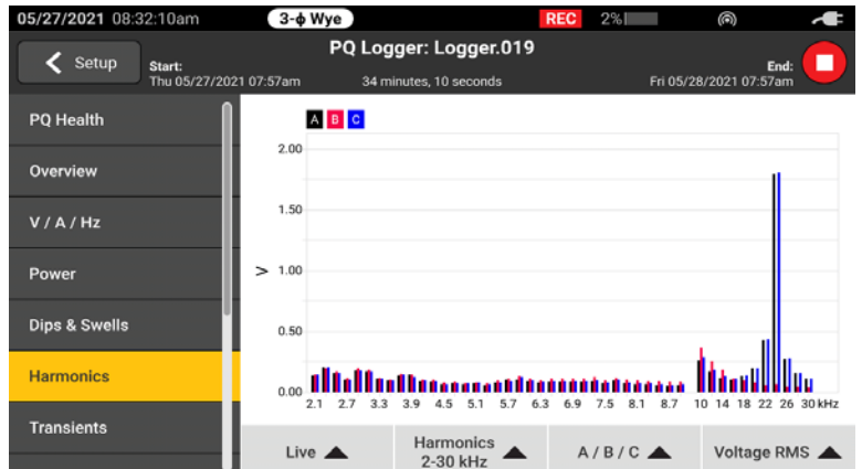
A full range of harmonics available on the Fluke 1775 and 1777 models are available from the first 100 integer harmonics and from 2 kHz to 30 kHz
