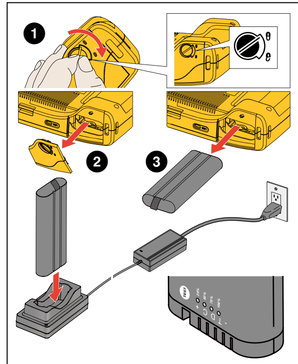
Figure 1. Battery
