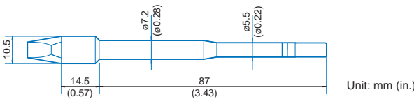
TX2-XD6 Shape-6XD
