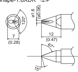
TX1-XDR16 Shape-1.6XDR
