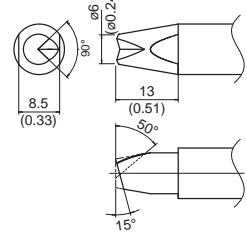
TX2-XRK Shape-XRK
