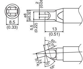
TX2-XRK Shape-XRK
