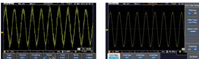
Unfiltered Waveform with Noise Interference
