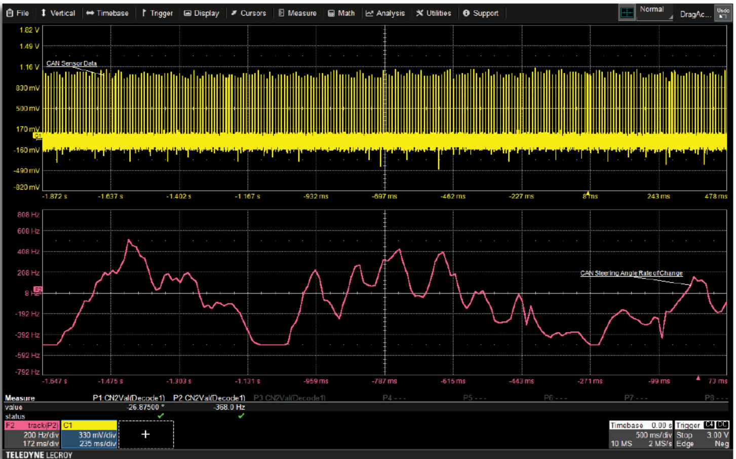
Shown above is a long acquisition of a CAN serial data signal (top waveform) that contains embedded digital data for steering wheel angle rate of change (deg/s, or Hz). The Message to Value parameter was configured to locate and extract the digital steering wheel angle range data from particular locations in specific CAN serial messages, and then converted from digital to analog form with proper re-scaling and physical units. The serial data DAC waveform (bottom waveform) is shown in the lower grid.
