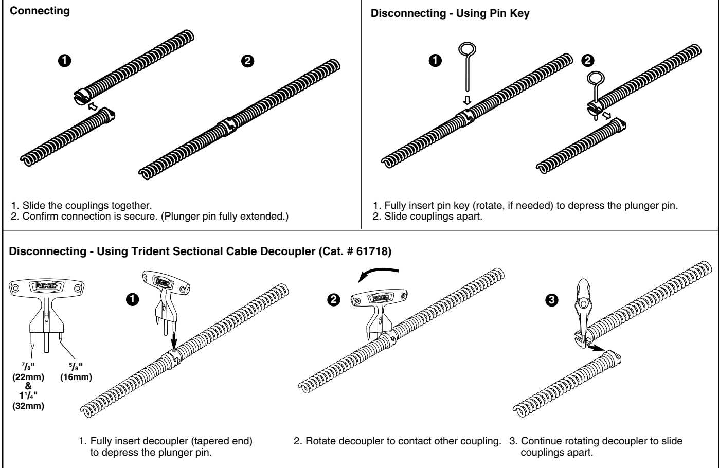
Figure 8 – Coupling and Uncoupling
