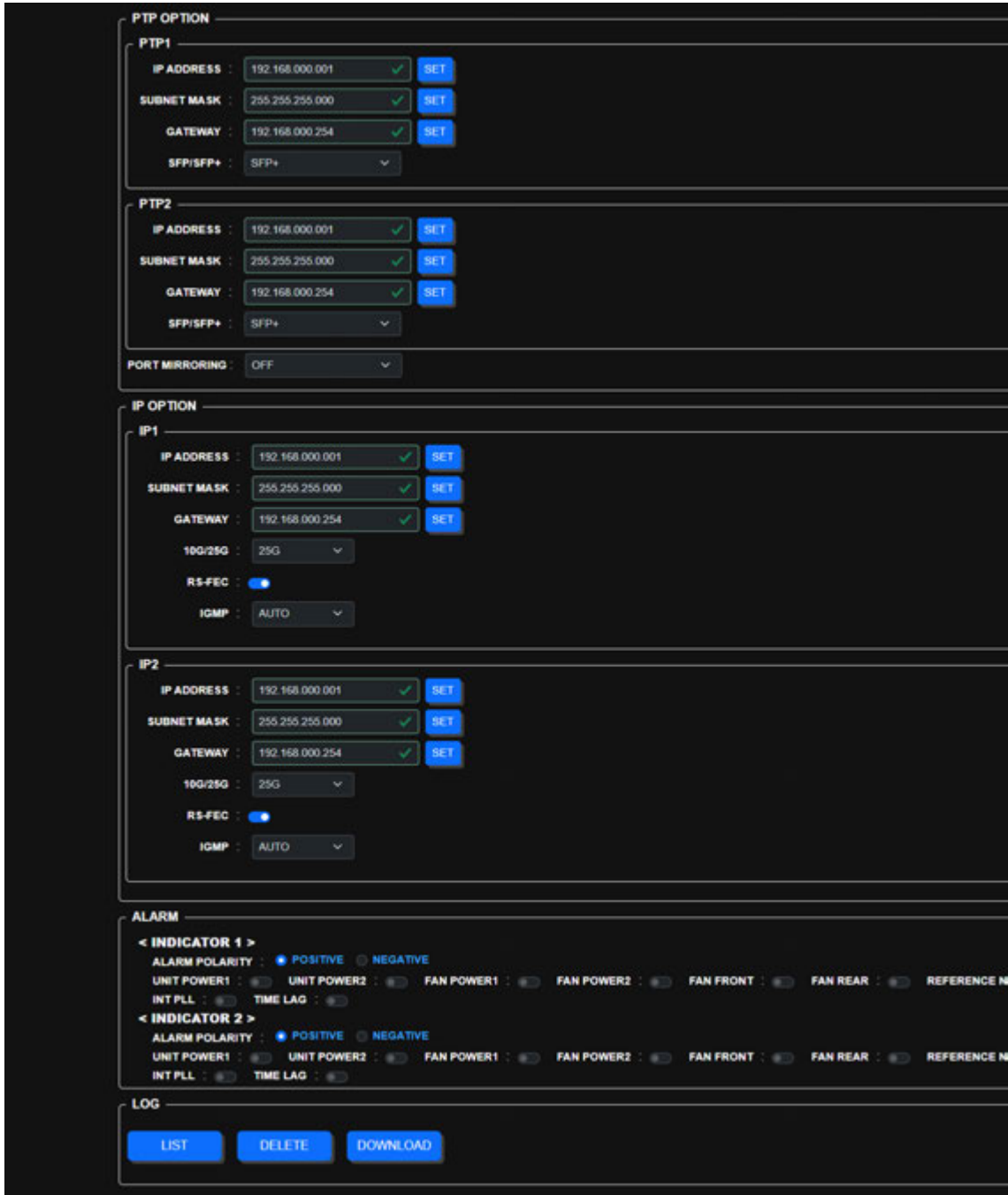
Figure 18-16 | SYSTEM screen
