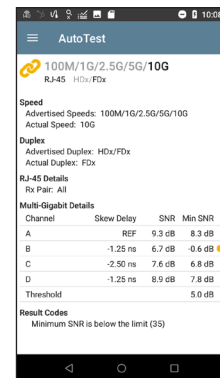
Cabling SNR measurement validates Multi-Gig links
