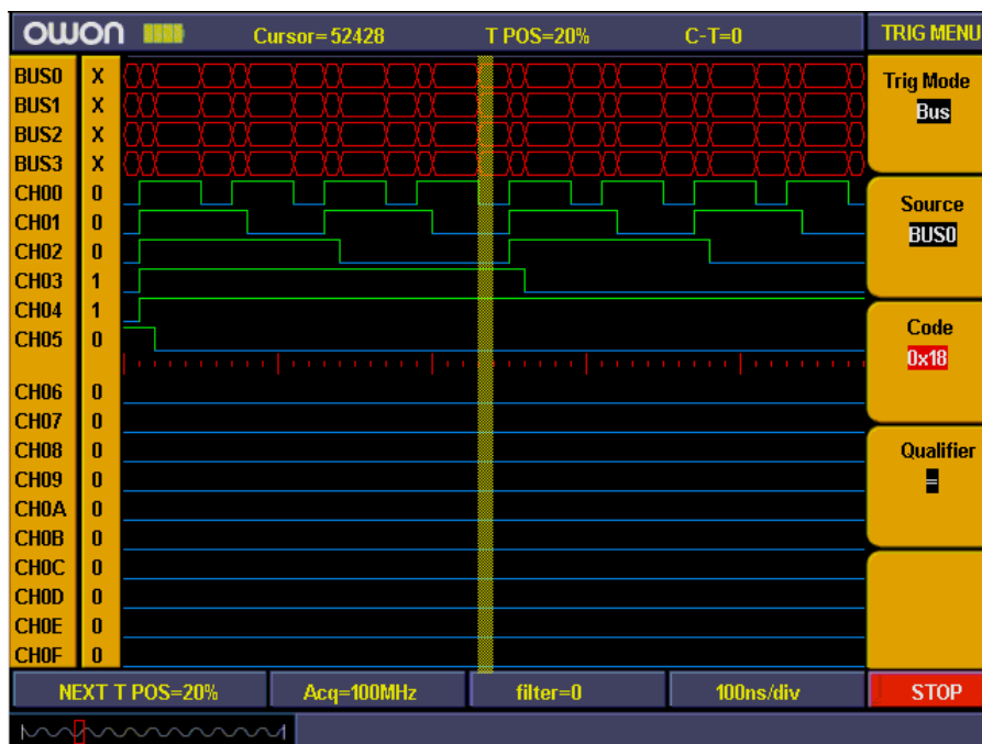
Fig.5-57: Bus trigger
