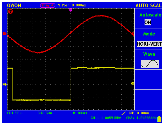
Fig.5-52 single cycle mode
