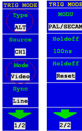
Fig.5-24 Alternate trigger(Trigger Type: video) Menu
