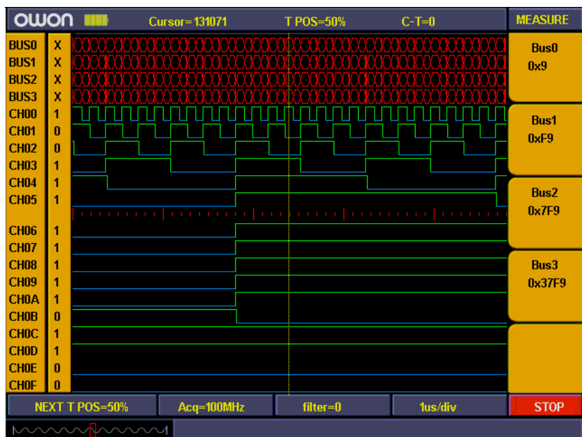
Fig.5-72: Bus measurement
