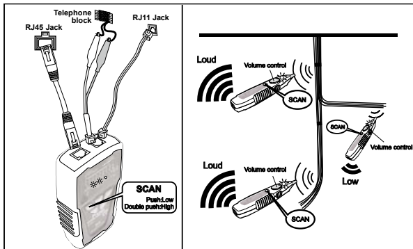
Figure 4 Isolating Cable
