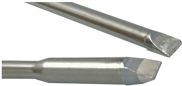
Comparing an HTD and an STTC tip of similar geometry.
