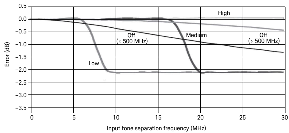
Figure 1. Flatness response.
