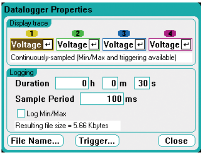
Figure 6. To set up the data logger, use a menu screen to select the operating parameters. Setup screens like this are used throughout the DC power analyzer.
