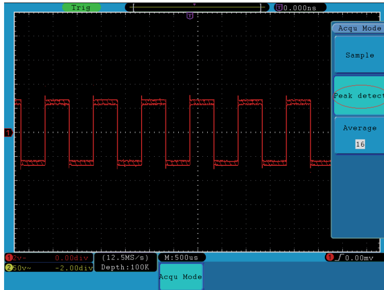
Figure 39. Peak Detect mode, under which the burrs on the falling edge of the square wave, can be detected and the noise is heavy.
