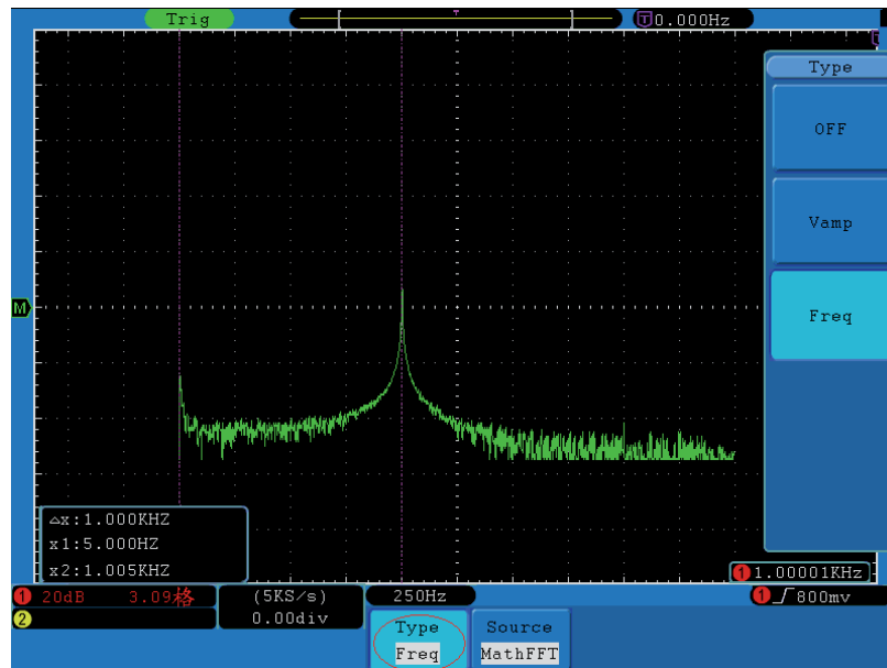
Figure 70. Wave of Freq cursor measurement.
