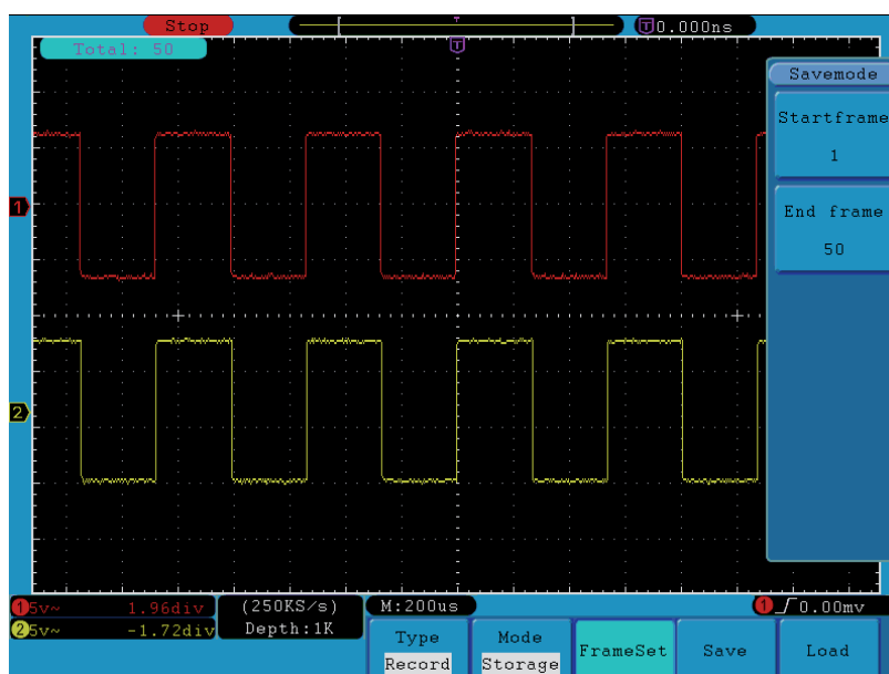
Figure 52. Wave Storage.
