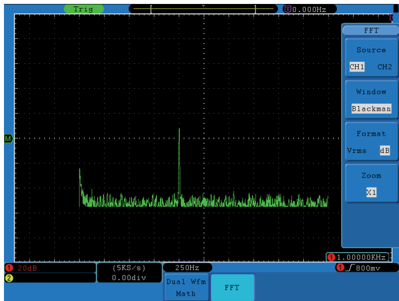
Figure 24. Blackman window.
