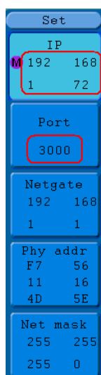
Figure 76. Set the network parameters of the oscilloscope.
