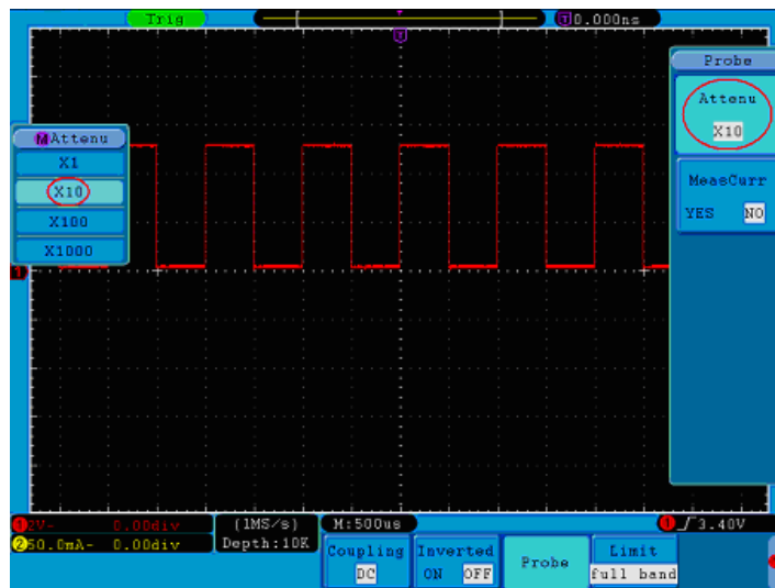
Figure 16. Regulation of the Attenuation Ratio of the Probe.
