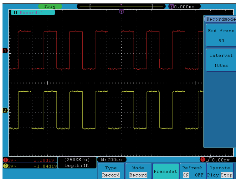
Figure 50. Wave Record.
