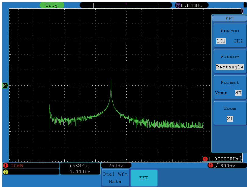
Figure 21. Rectangle window.
