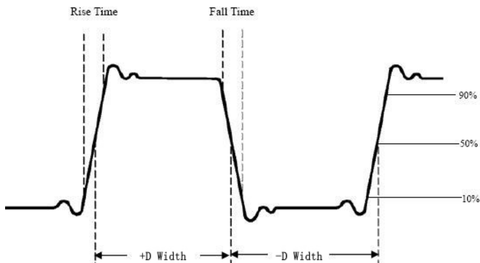
Figure 64. Shows a pulse with some of the time measurement points.
