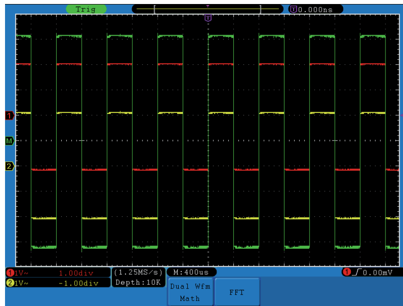
Figure 20. Waveform resulted from CH1 +CH2.
