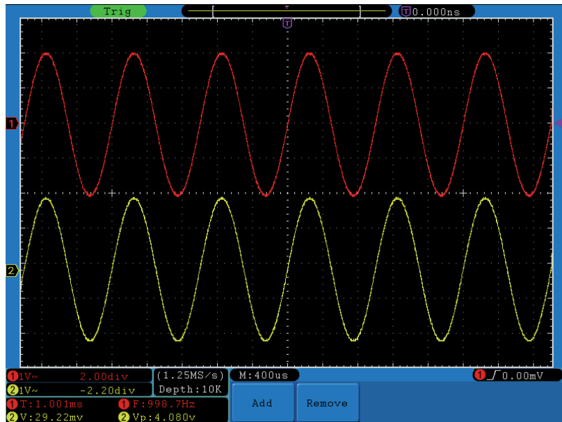
Figure 80. Measure Frequency and PK-PK value for a given signal.
