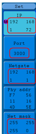
Figure 79. Set the network parameters of the oscilloscope.
