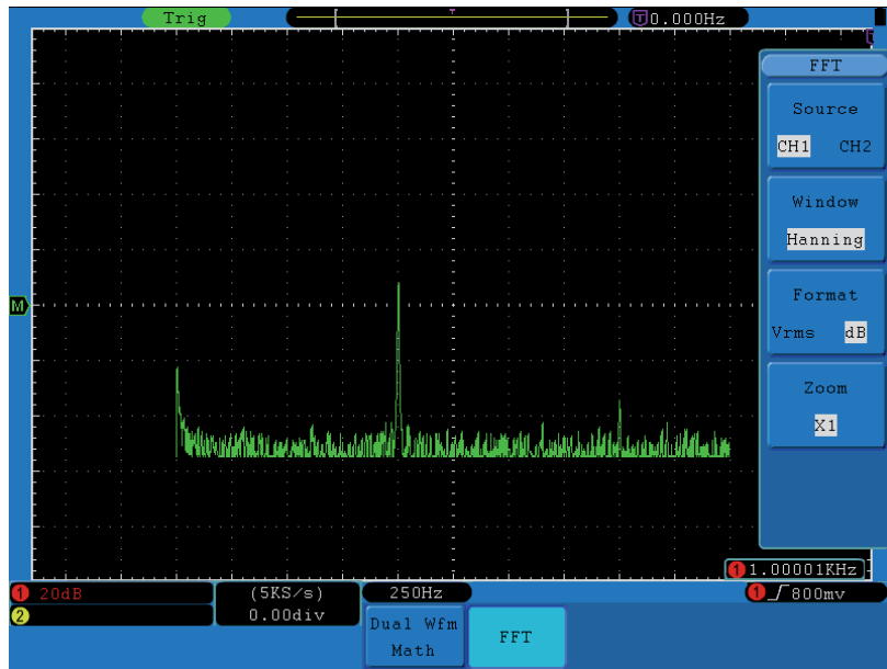
Figure 23. Hanning window.
