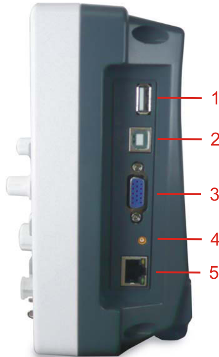
Figure 2. Right Side Panel
