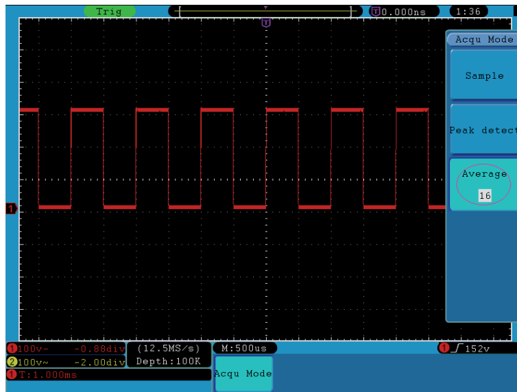
Figure 41. The displayed waveform after the noise is removed under the Average Mode, in which the average number of 16 is set.
