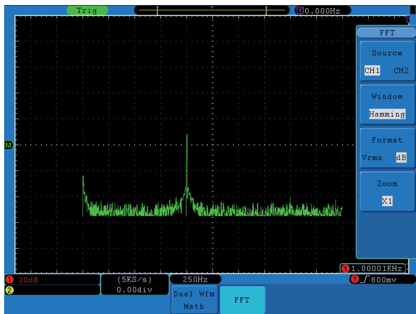
Figure 22. Hamming window.
