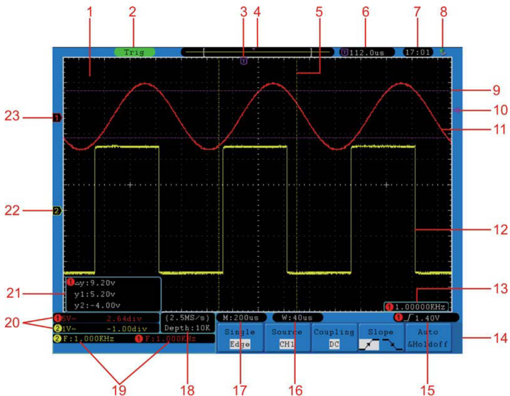
Figure 5. Illustrative Drawing of Display Interfaces (take OD-603) for instance)
