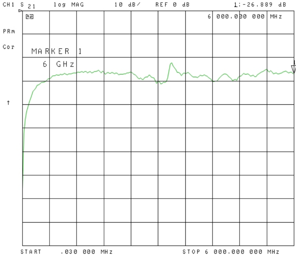
Image 6 - H10 coupling loss, 30 kHz to 6 GHz, lin.
