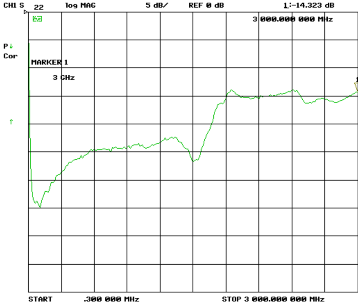
Image 15 - Wideband amplifier output return loss, IS221 300 kHz to 3 GHz lin.
