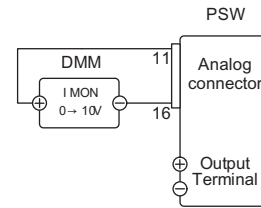
External DMM Monitoring of the Output Current
