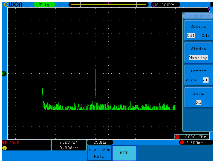
Fig.5-10 Hanning window
