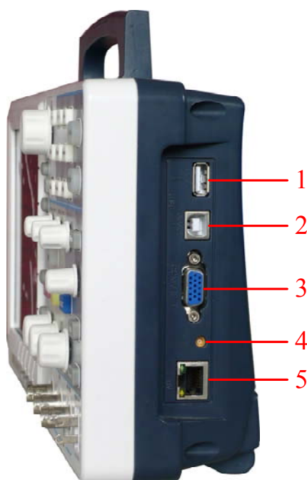
Fig. 4-2 Right side panel
