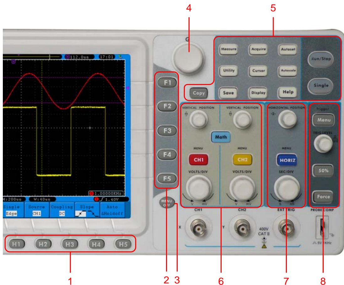
Fig. 4-4 Keys Overview
