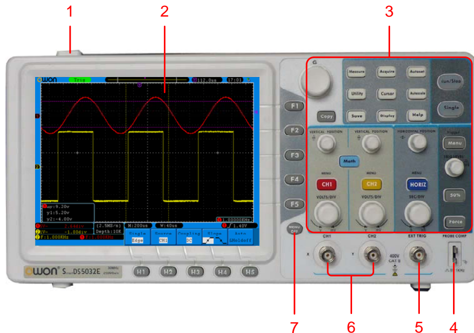
Fig. 4-1 Front panel
