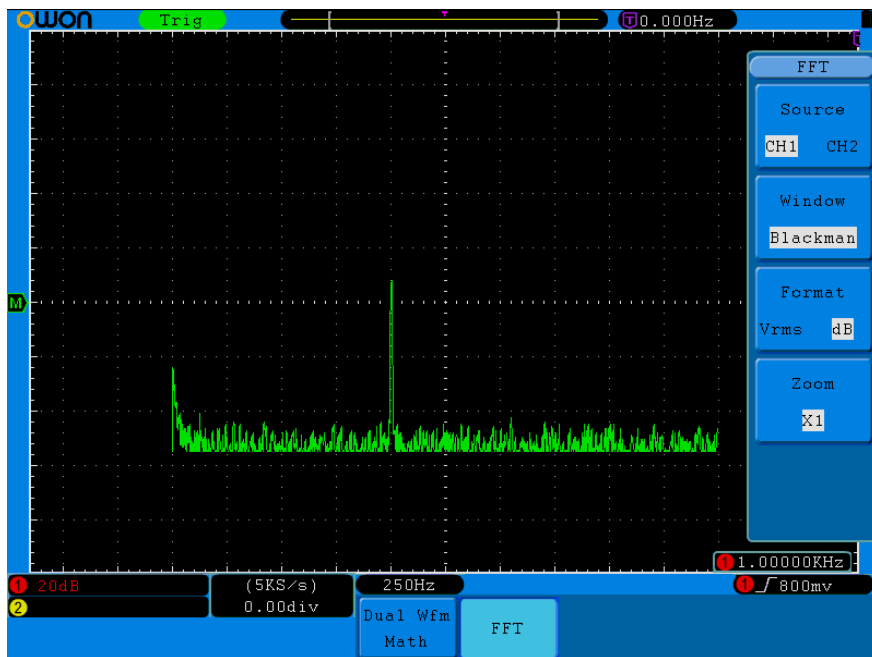
Fig.5-11. Blackman window
