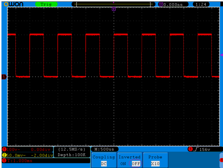
Fig. 5-4 Original Waveform
