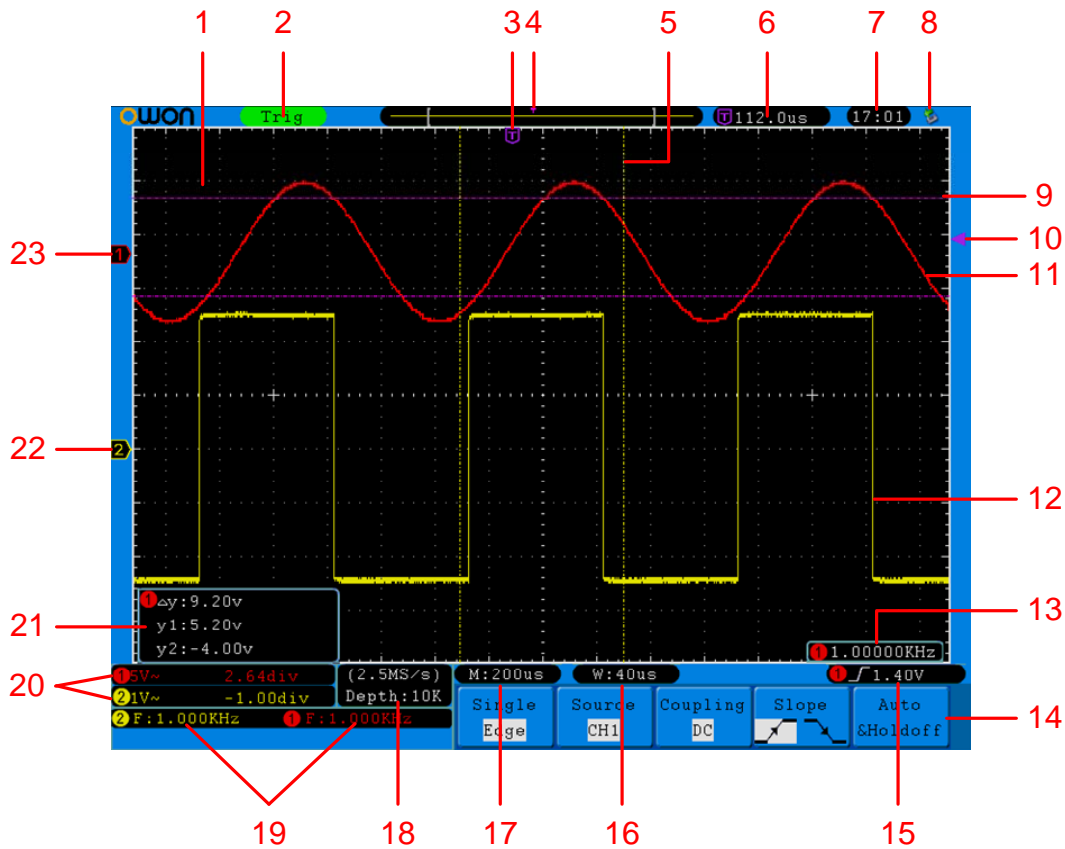
Fig. 4-5 Illustrative Drawing of Display Interfaces
