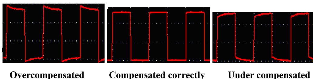
Fig. 4-7 Displayed Waveforms of the Probe Compensation
