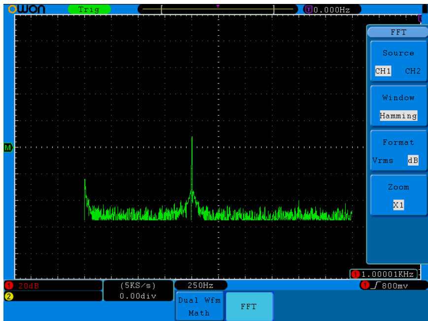
Fig.5-9 Hamming window
