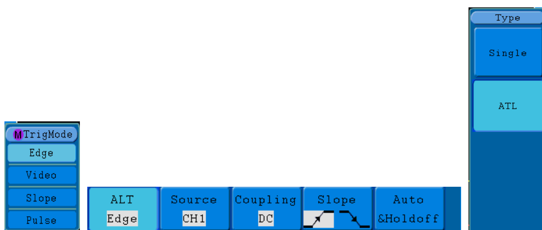
Figure 5-22 Alternate trigger (Trigger Type: Edge) Menu
