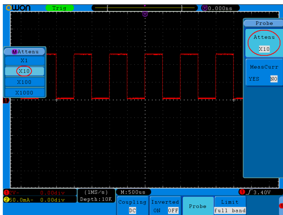
Figure 5-3 Regulation of the Attenuation Ratio of the Probe
