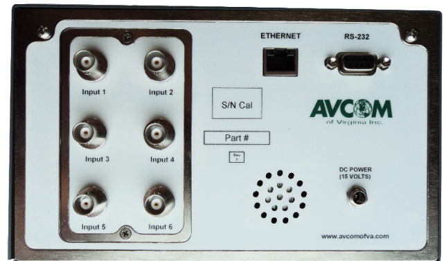
(Rear view of SNG-2500C-6BL)
