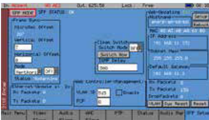
Sx TAG IP with SFP Setup
