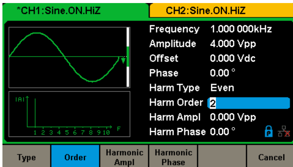
Figure 2-20 Harmonic Interface
