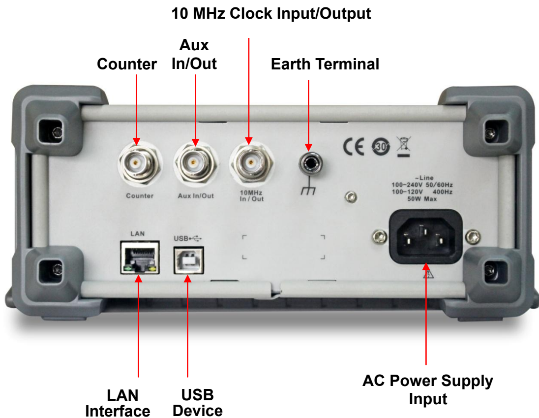
Figure 1-3 Rear Panel
