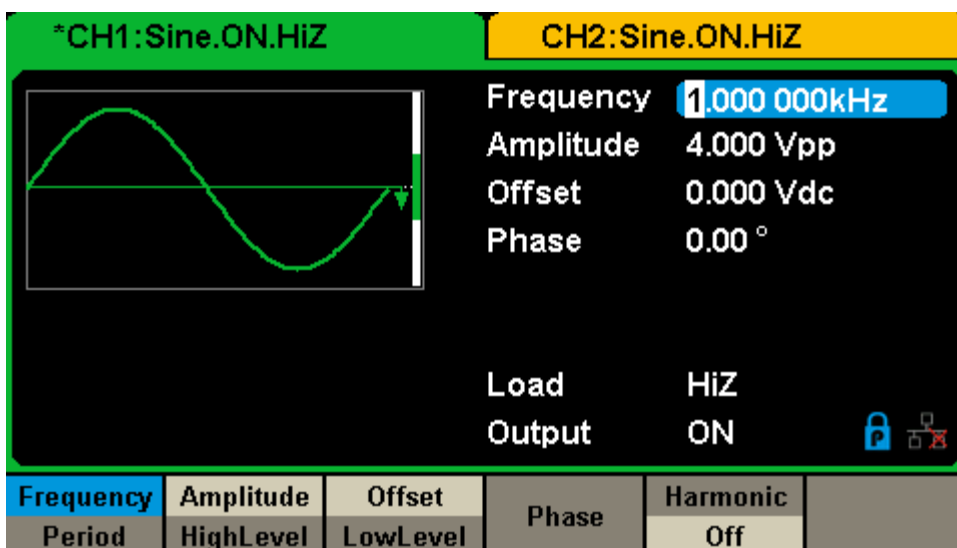
Figure 2-71 Phase-locked Mode
