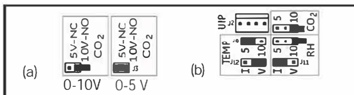
Jumper Settings for Non-Display (a) and Display (b) Units
