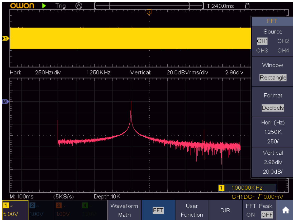
Figure 4-25 Rectangle window
