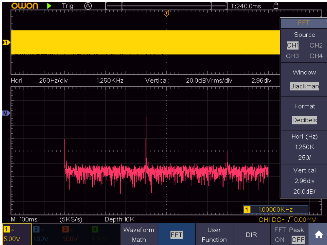
Figure 4-26 Blackman window
