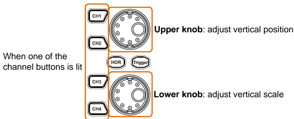
Figure 3-10 Vertical Control
