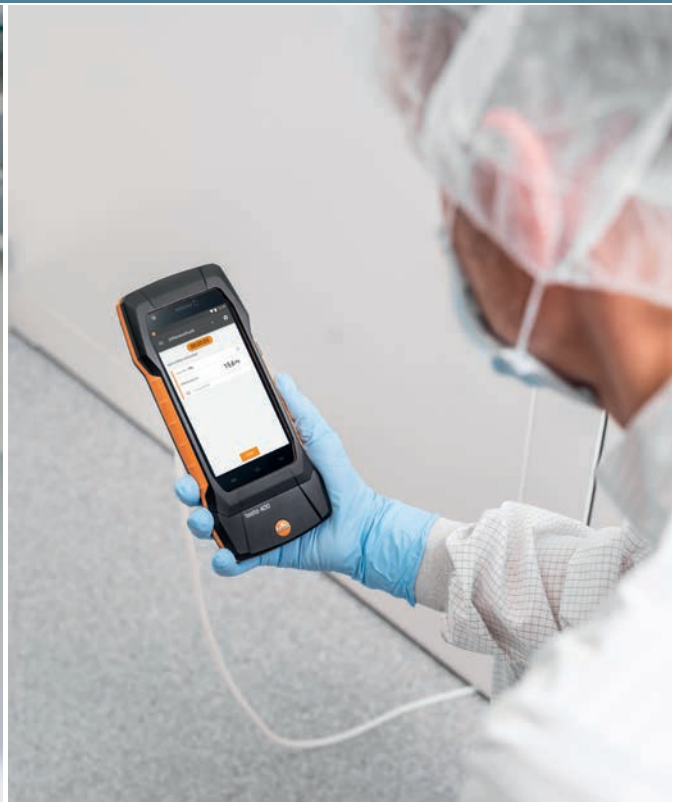
The differential pressure sensor of the testo 400 fulfils the accuracy requirements of ISO 14644.
