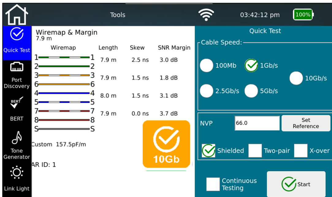
Figure 51 - Wiremap & Margin
