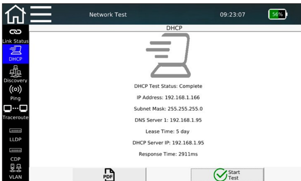
Figure 44 - DHCP test
