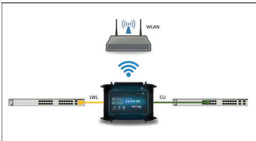
Figure 42 - Test setup for connecting to an active network
