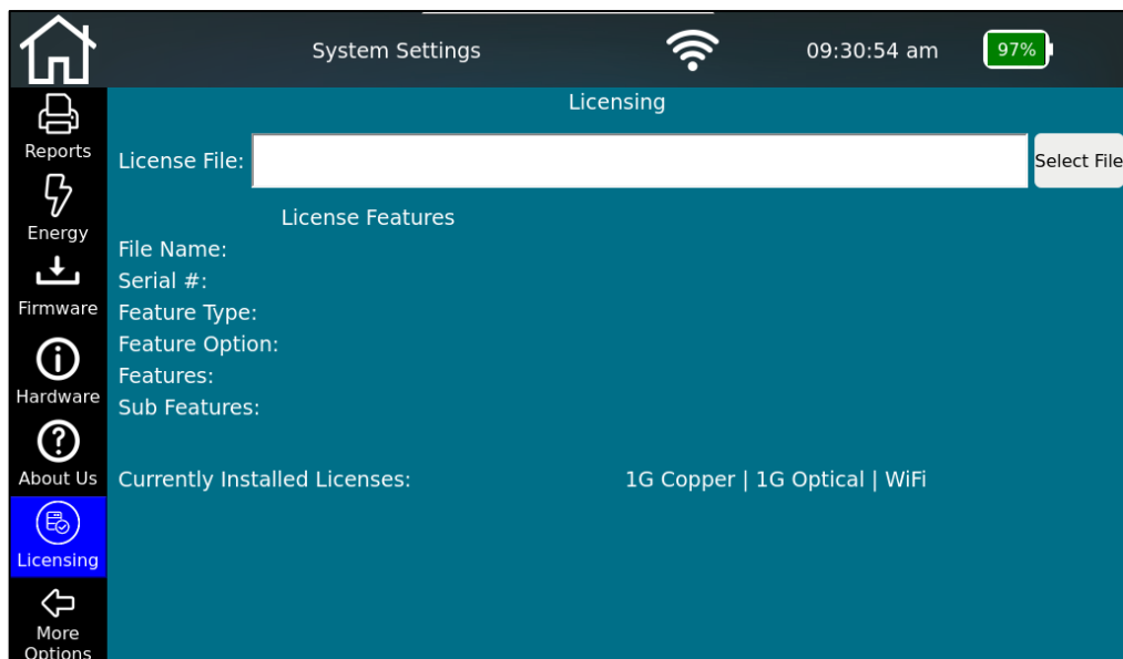
Figure 22 - License management
