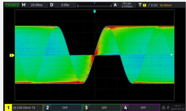
Use the original Ultra Phosphor technique to display the waveform details.
