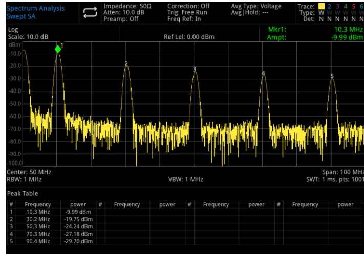
Figure 4-3 Peak List
