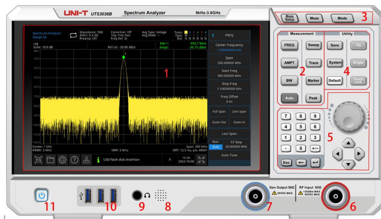
Figure 1-1 Front Panel
