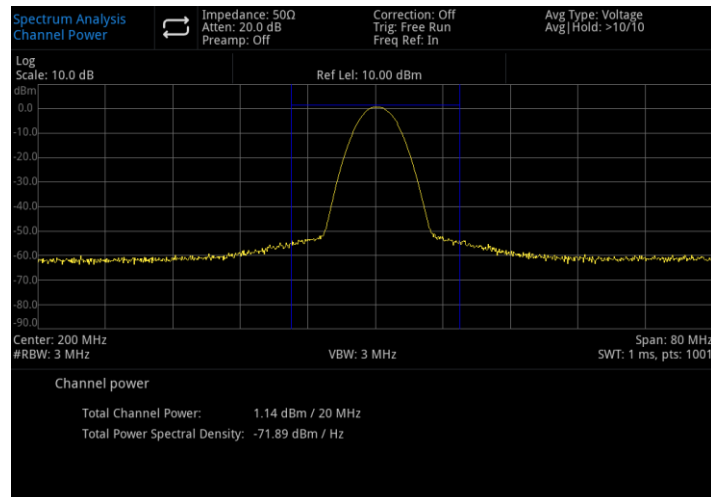
Figure 5-1 Channel Power
