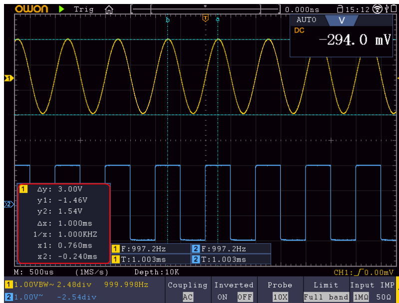
Figure 4-23 Time&Voltage Cursor Measurement
