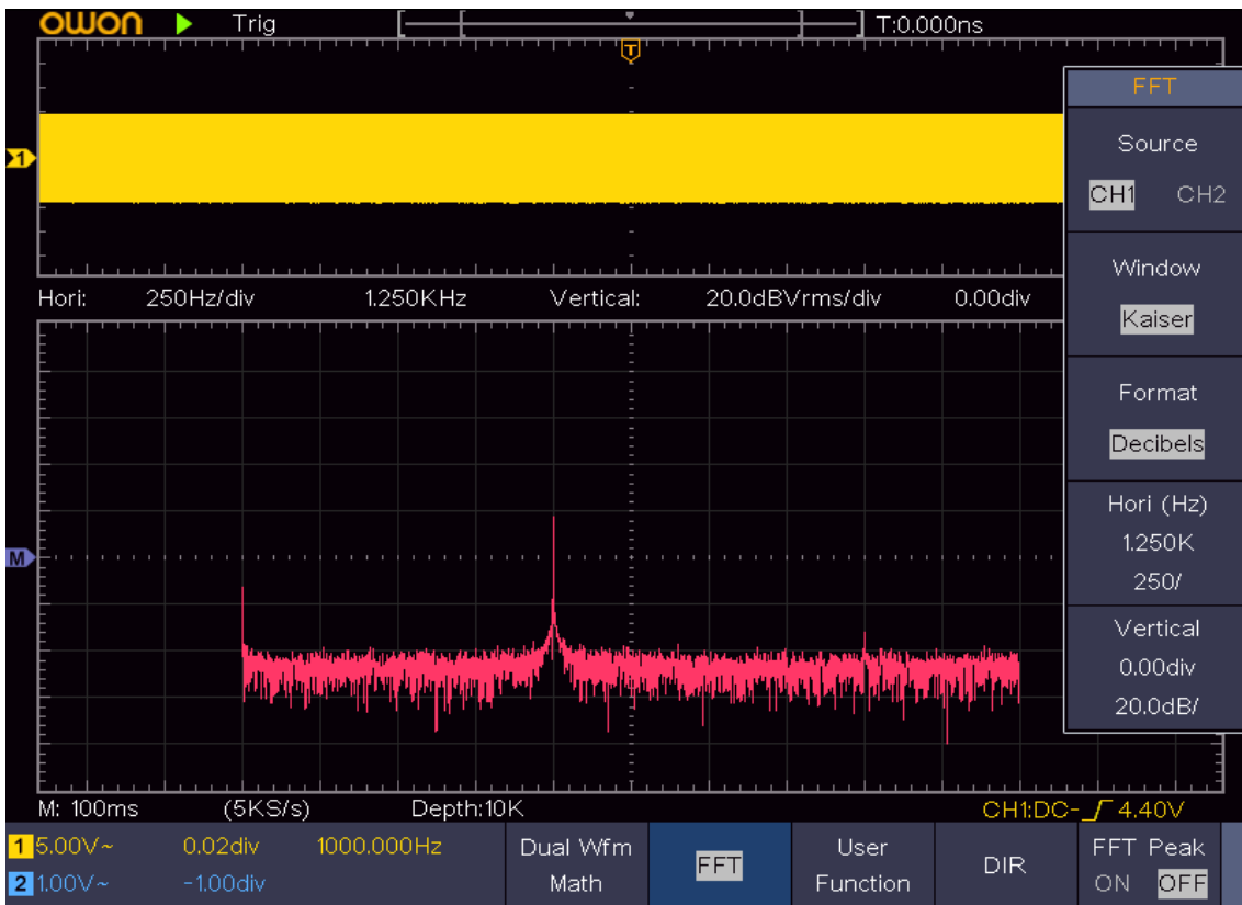
Figure 4-5 Kaiser window
