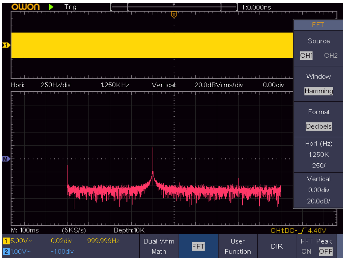
Figure 4-1 Hamming window
