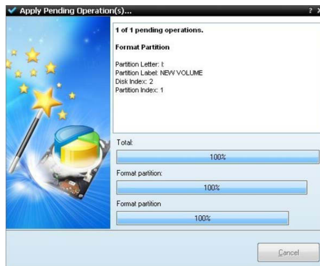
Figure 4-17: Format process
