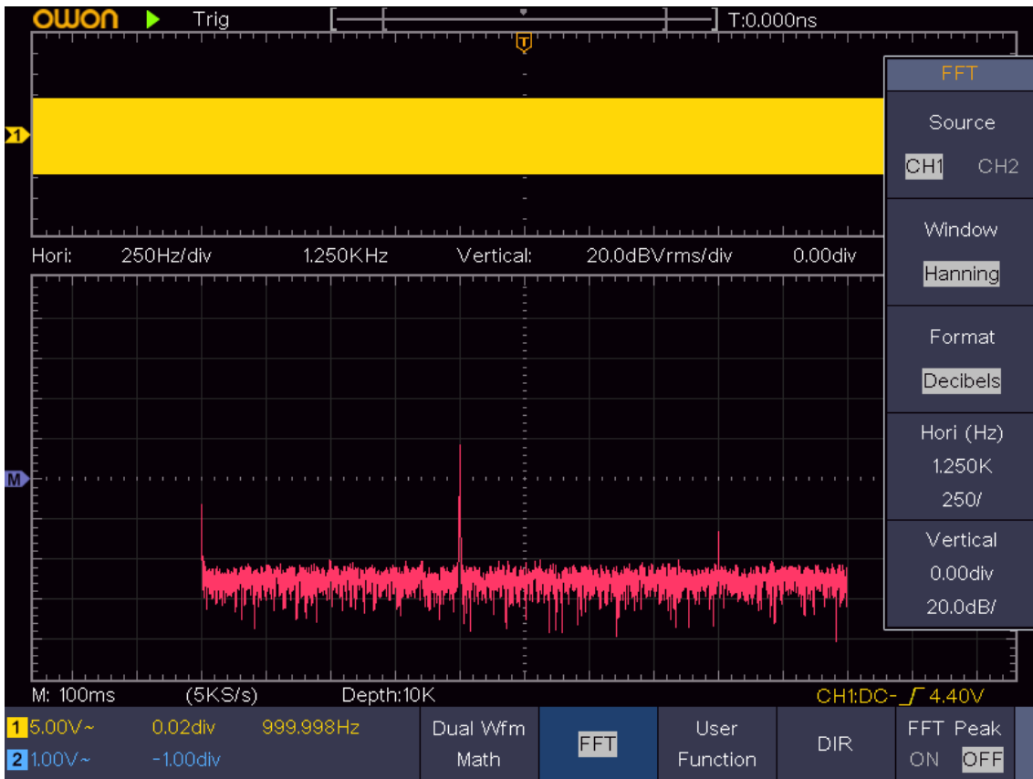
Figure 4-4 Hanning window
