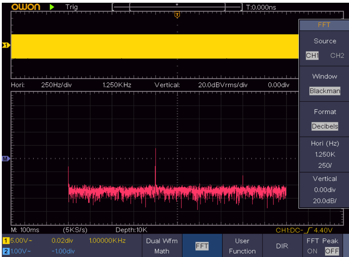
Figure 4-3 Blackman window
