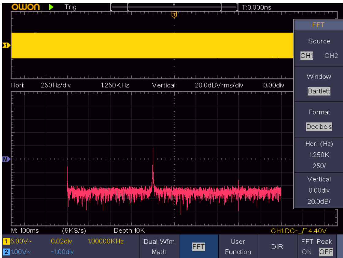
Figure 4-6 Bartlett window
