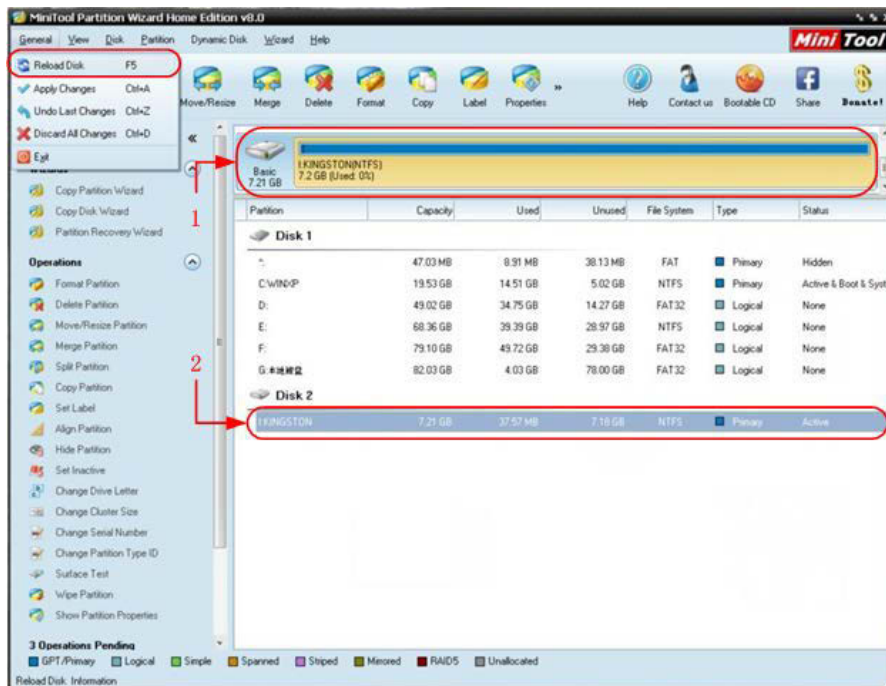
Figure 4-13: Reload Disk
