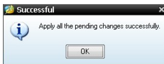
Figure 4-18: Format successfully
