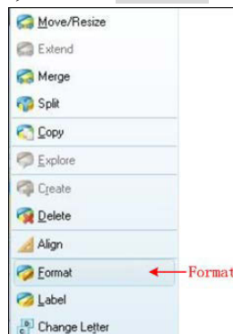
Figure 4-14: Choose format
